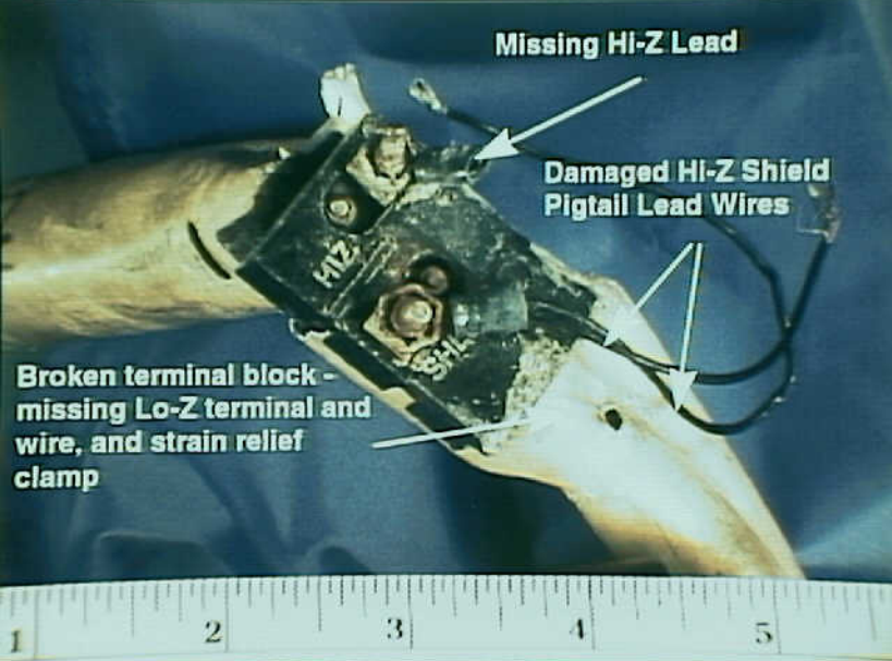
Systems 9 - Exhibit No. 9B - Photo 18. Figure 18g. Representative damage to a fuel probe, wiring and terminal block from N93119.
