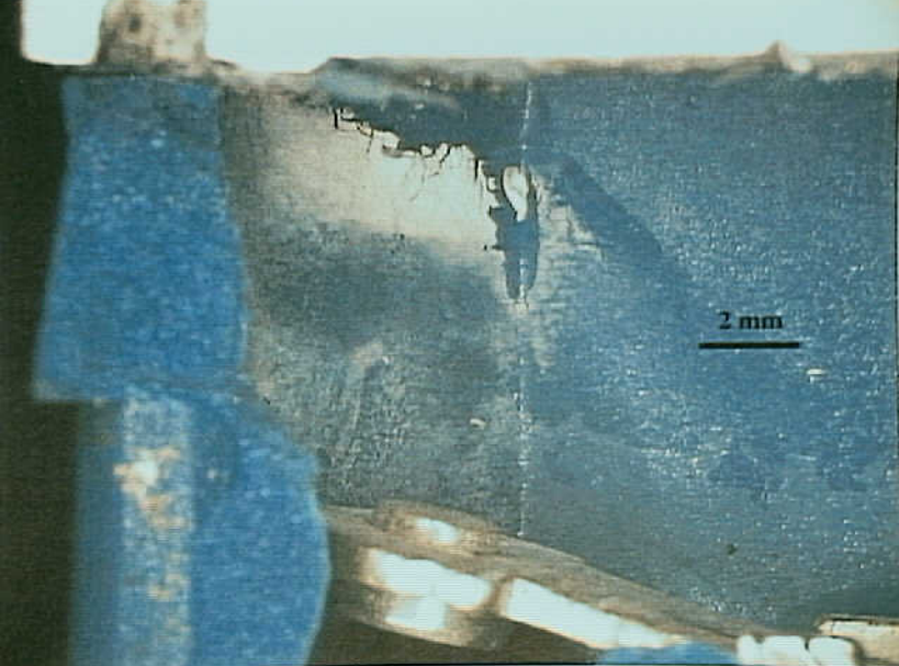
Systems 9 - Exhibit No. 9B - Photo 18. Figure 18a. Evidence of internal salt water-like deposits on the scavenger pump switch case near the contact.
