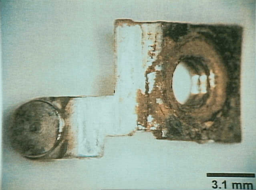
Systems 9 - Exhibit No. 9B - Photo 17. Figure 17c. The stationary line terminal and contact of the RTV circuit breaker have a tarnished appearance.
