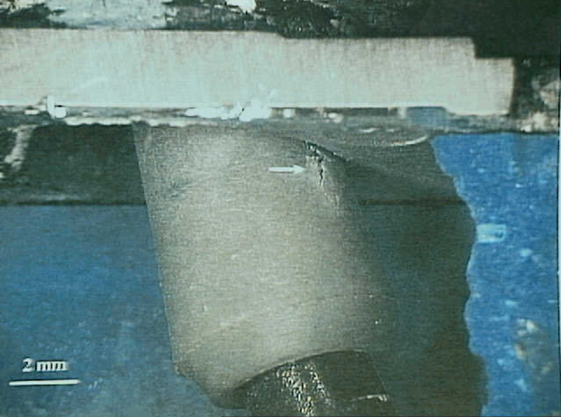
Systems 9 - Exhibit No. 9B - Photo 16. Figure 16a. Scavenge pump switch plunger guide exhibiting surface cracks from the mold runner (arrow).
