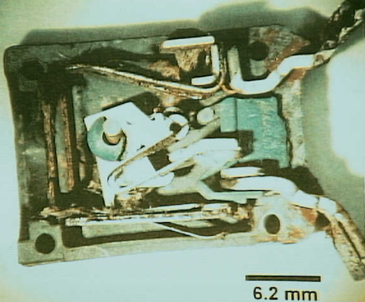
Systems 9 - Exhibit No. 9B - Photo 15. Figure 15c. The various mechanical components of the RTV circuit breaker are corroded. The moving contacts are lying against the stationary contacts.
