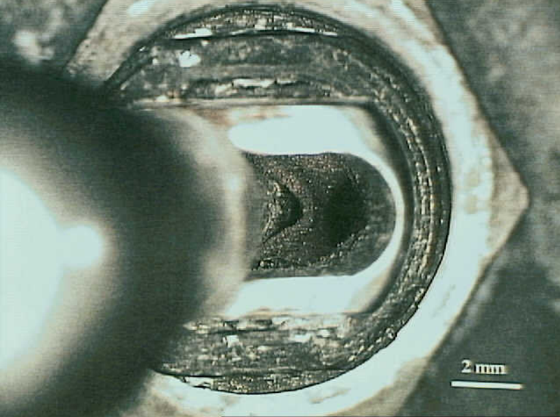
Systems 9 - Exhibit No. 9B - Photo 15. Figure 15a. The environmental seal sleeve was displaced from the knob towards the "on" position.
