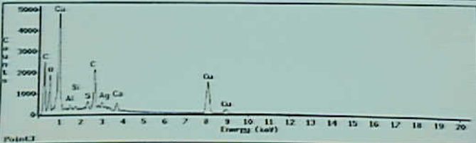
Systems 9 - Exhibit No. 9B - Photo 13. Figure 13g-2. Elemental X-ray microanalysis of damaged Hi-Z shield pigtail lead wire from N93119. Note presence of copper and silver on PTFE insulation at sites 1 and 2.
