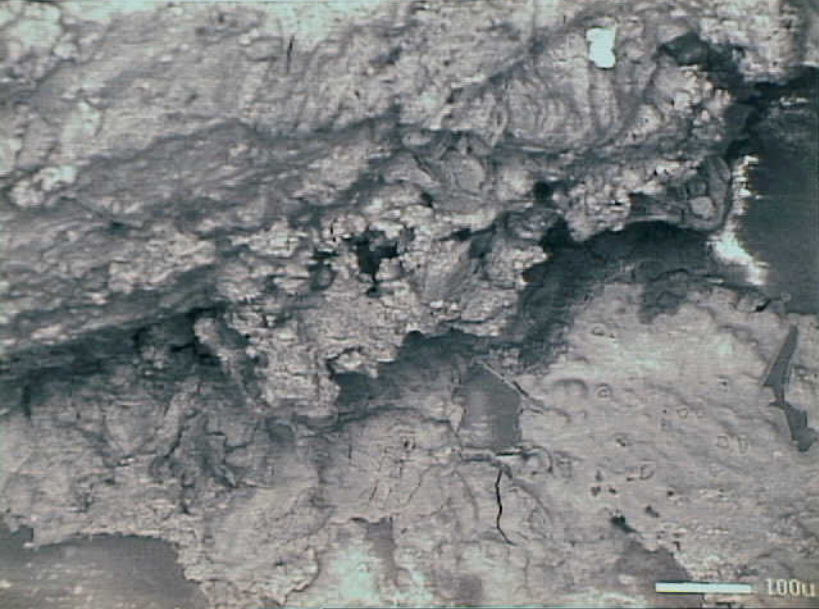
Systems 9 - Exhibit No. 9B - Photo 13. Figure 13b. Base of the feedthrough pin and glass to metal seal of N.O. contact A1.
