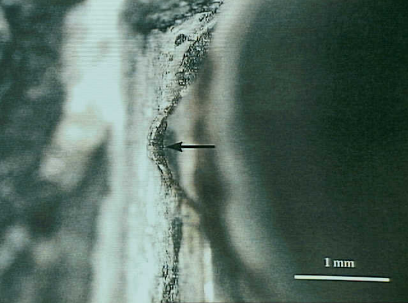
Systems 9 - Exhibit No. 9B - Photo 13. Figure 13a. Close-up showing the lip shaped metal displacement of the locking cam (arrow).
