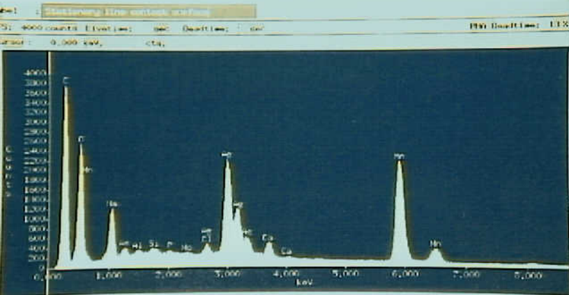
Figure 12. EDS spectrum of a area described as being tarnished on the stationary line contact of the SPR circuit breaker. The silver in both spectrums is primarily from the
