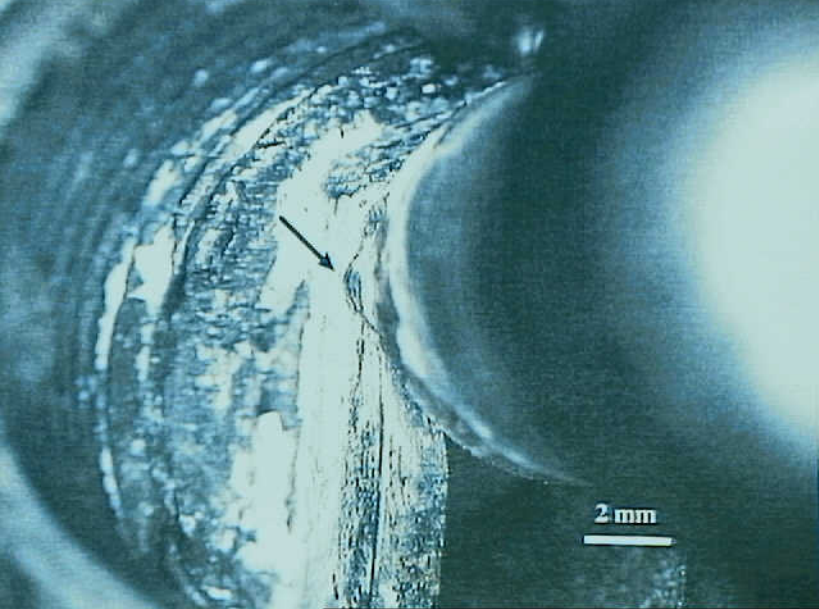
Systems 9 - Exhibit No. 9B - Photo 12. Figure 12a. Scavenge pump knob exhibiting displacement towards the right side of the locking cam (left in the photograph).
