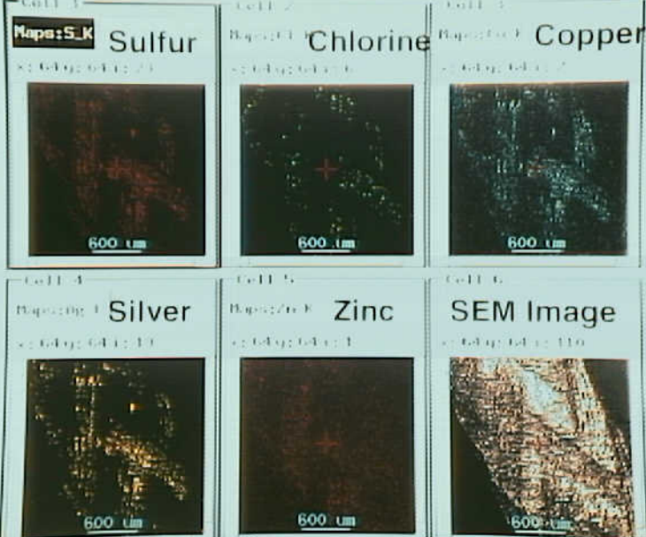
Systems 9 - Exhibit No. 9B - Photo 11. Figure 11g. EDS elemental X-ray map of wire insulation surface in Figure 10. Note the distribution of copper, silver, and sulfur.
