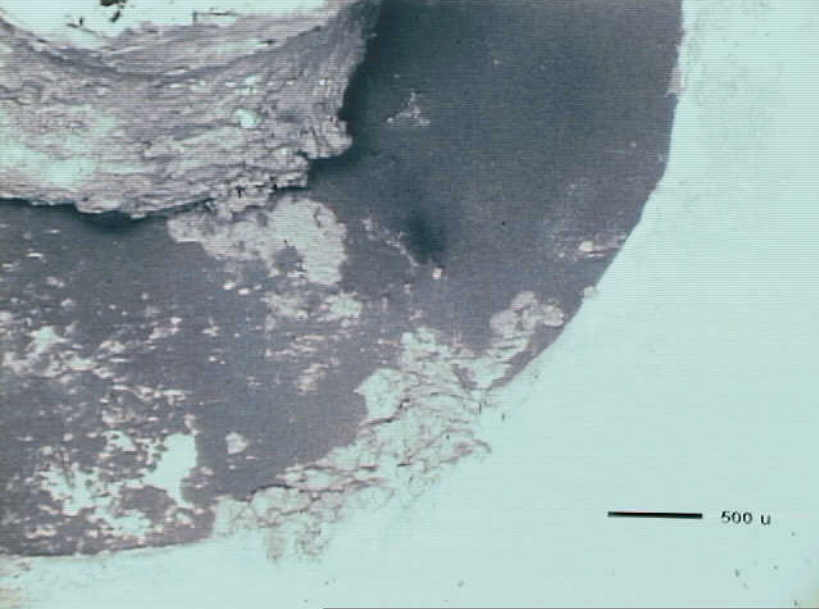
Systems 9 - Exhibit No. 9B - Photo 11. Figure 11b. The glass to metal seal area of N.O. contact A1 after the residue was brushed away.
