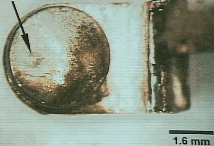
Systems 9 - Exhibit No. 9B - Photo 10. Figure 10c. The stationary load contact of the SPR circuit breaker has a tarnished appearance. Arrow highlights the mechanical wear from the making and breaking of the contacts.
