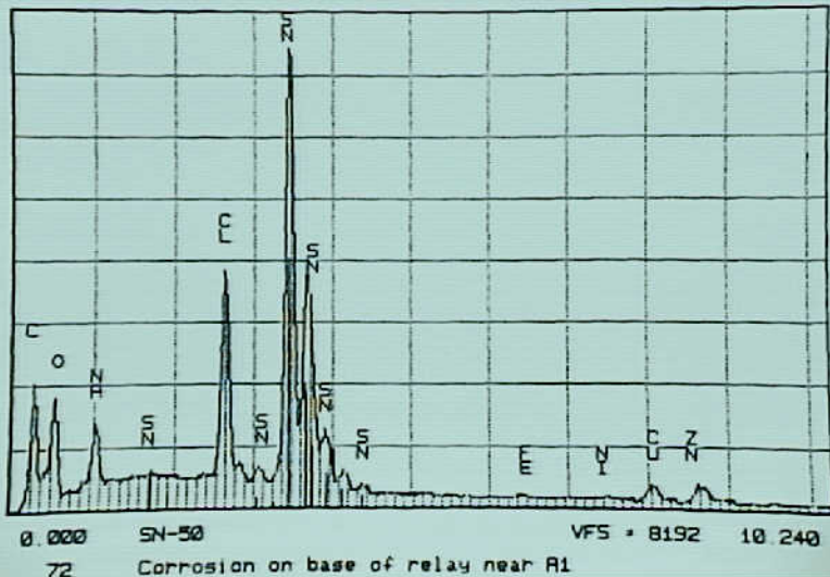
Systems 9 - Exhibit No. 9B - Photo 10. Figure 10b. Corrosion products on base of relay near A1.
