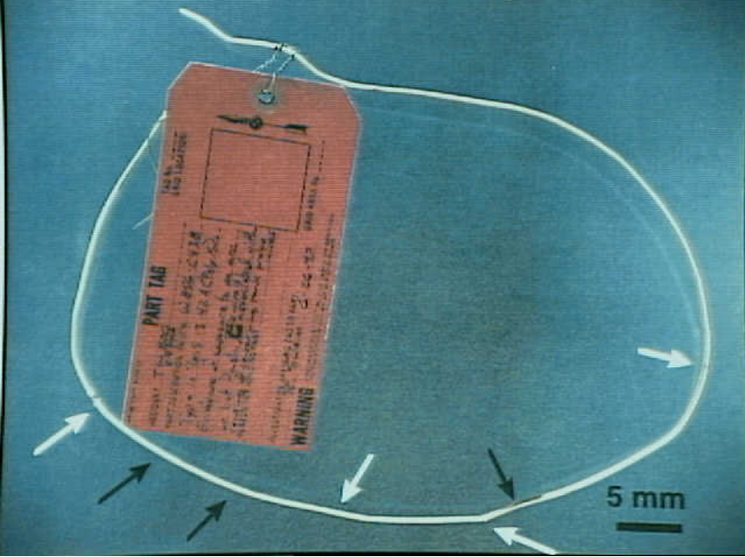
Systems 9 - Exhibit No. 9B - Photo 1. Figure 1d. Wire sample submitted for analysis. The insulation exhibited blacked areas (black arrows) and mechanical damage (white arrows).
