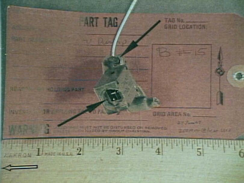
Systems 9 - Exhibit No. 9B - Photo 1. Figure 1c. As received condition of the SPR circuit breaker. The upper arrow highlights the corroded terminal hardware. The lower arrow highlights the missing actuator stem and mounting bushing.
