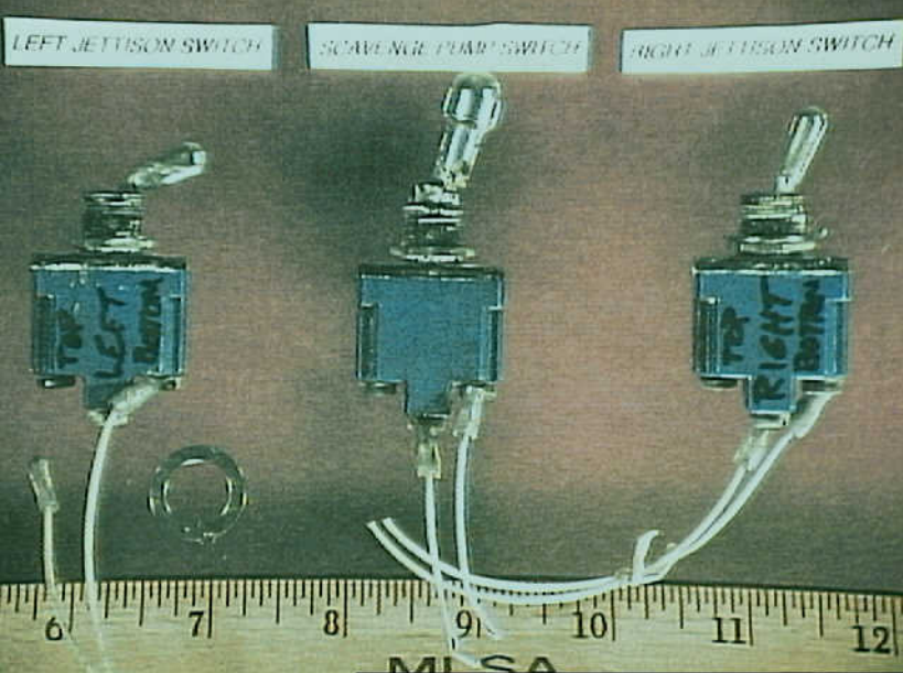
Systems 9 - Exhibit No. 9B - Photo 1. Figure 1a. Side 1 of the three switches received for analysis.
