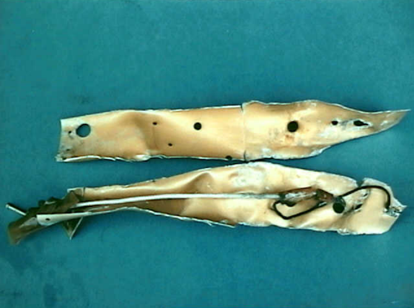
Systems 9 - Exhibit No. 9A - Addendum 1 - (Fuel Probes) Photo 6. Fragment 80 Compensator inner
