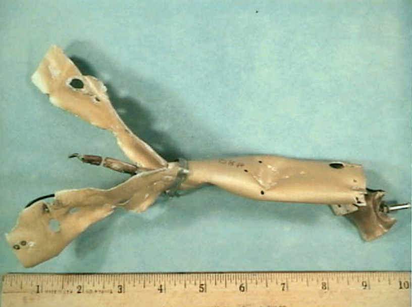
Systems 9 - Exhibit No. 9A - Addendum 1 - (Fuel Probes) Photo 4. Fragment 80 Compensator after parting flattened upper third.
