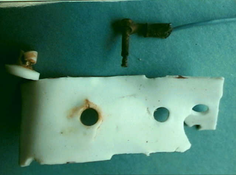
Systems 9 - Exhibit No. 9A - Addendum 1 - (Fuel Probes) Photo 18. Fragment 80 Compensator terminal block teflon insulator, tube face.
