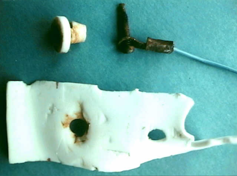
Systems 9 - Exhibit No. 9A - Addendum 1 - (Fuel Probes) Photo 17. Fragment 80 Compensator terminal block teflon insulators, exterior (terminal block) face.
