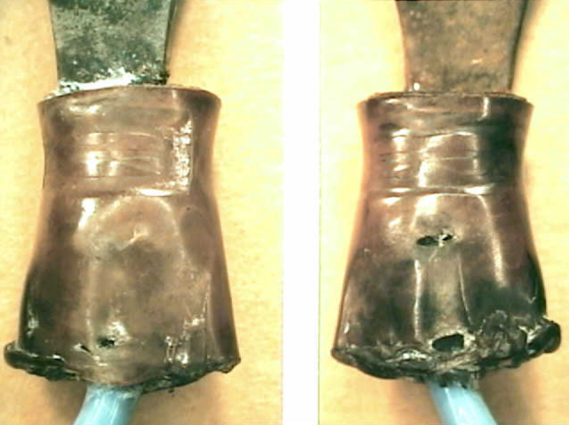
Systems 9 - Exhibit No. 9A - Addendum 1 - (Fuel Probes) Photo 15. Fragment 80 Compensator internal upper LO-Z ring connector with blackened and deformed lower plastic features. Left photo faces head of screw.
