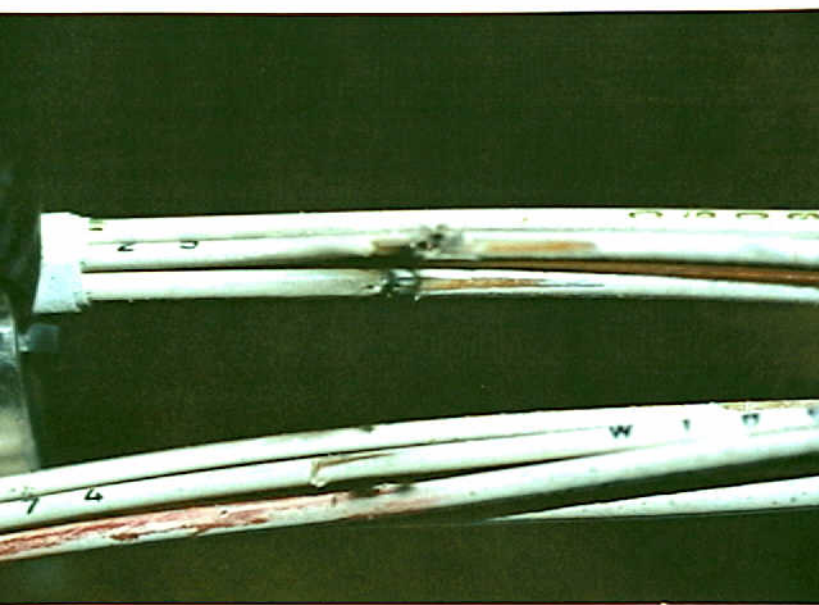
Systems 9 - Electrical Short Circuit/Arcing of Aged Aircraft Wiring - Figure 42. Test 17: Damage to wire bundle in the area of the flash..
