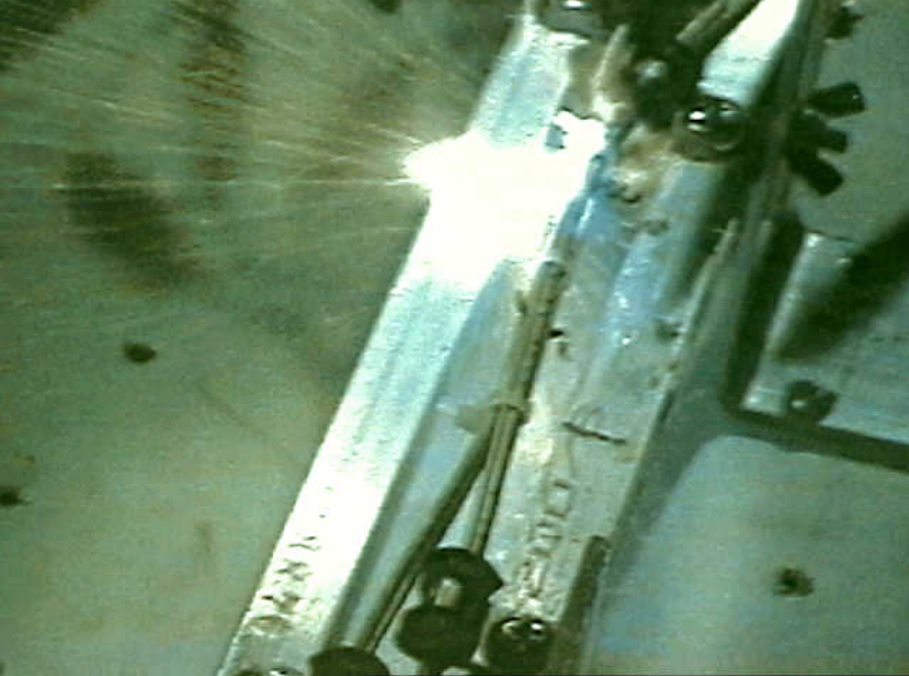
Systems 9 - Electrical Short Circuit/Arcing of Aged Aircraft Wiring - Figure 41. Test 17: Flash event during the longitudinal abrasion test.
