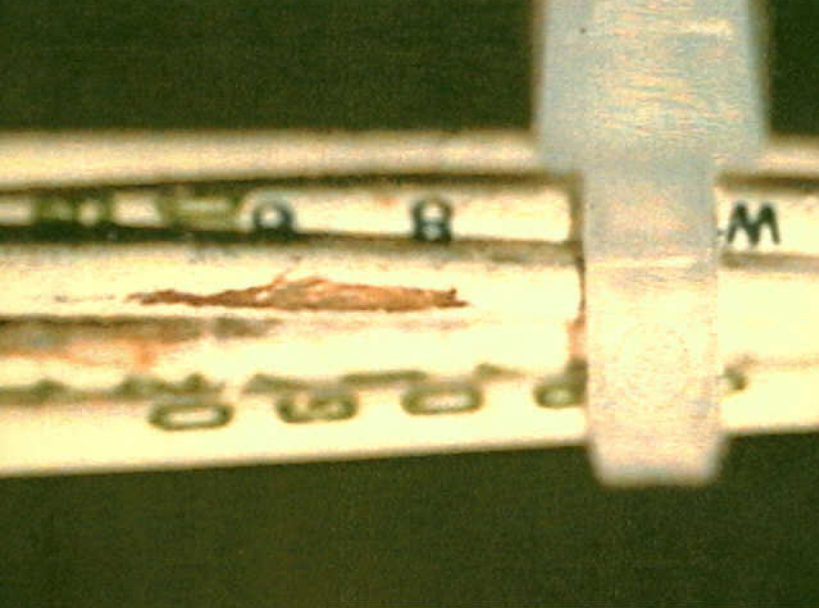
Systems 9 - Electrical Short Circuit/Arcing of Aged Aircraft Wiring - Figure 40. Test 17: Abrasion damage that did not reach to the conductor.
