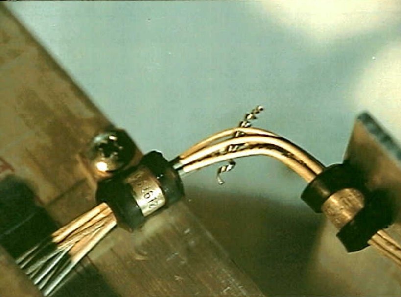
Systems 9 - Electrical Short Circuit/Arcing of Aged Aircraft Wiring - Figure 38. Test 16 A: Sample during the metal shaving abrader test 90 degrees (right angle)..
