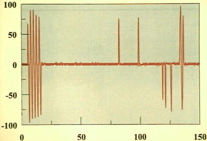
Systems 9 - Electrical Short Circuit/Arcing of Aged Aircraft Wiring - Figure 36. Test 12: Oscillogram of intermittent current during a flash event..
