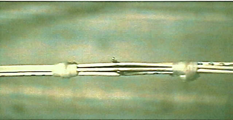
Systems 9 - Electrical Short Circuit/Arcing of Aged Aircraft Wiring - Figure 35. Test 12: Sample bundle after the flash shown in Figure 34..
