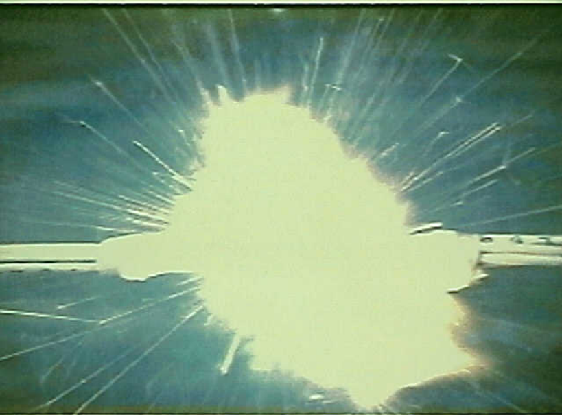
Systems 9 - Electrical Short Circuit/Arcing of Aged Aircraft Wiring - Figure 34. Test 12: Flash event during a metal shavings short circuit test..
