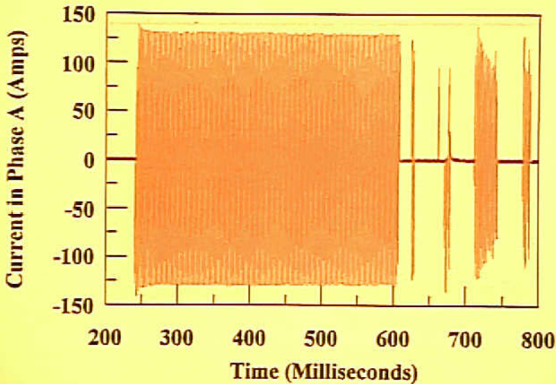
Systems 9 - Electrical Short Circuit/Arcing of Aged Aircraft Wiring - Figure 33. Test 9: Oscillogram of short circuit current that turns into intermittent arcing.
