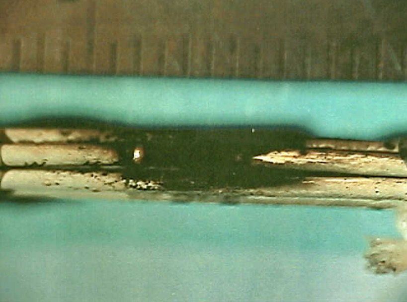
Systems 9 - Electrical Short Circuit/Arcing of Aged Aircraft Wiring - Figure 32. Test 6: Sample bundle after wet arc track testing with lavatory waste water for 10
