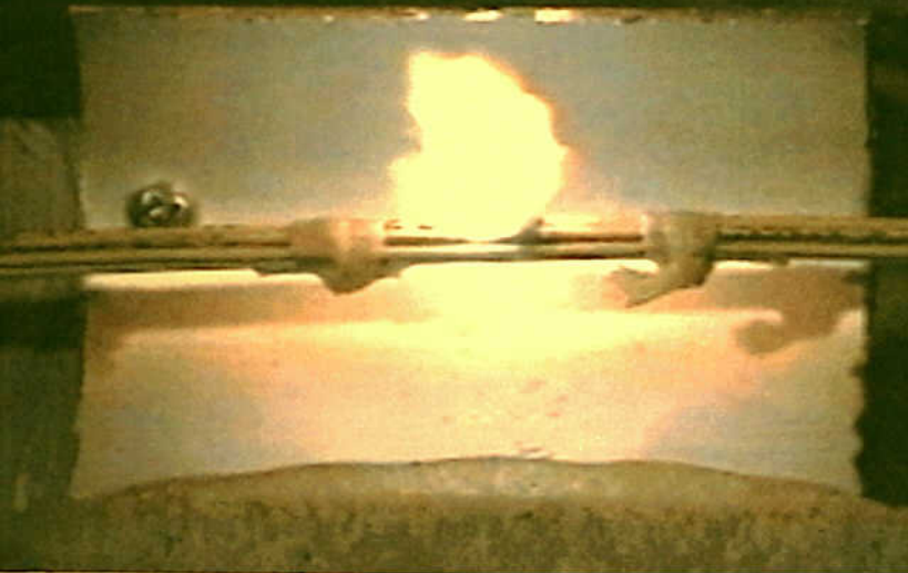
Systems 9 - Electrical Short Circuit/Arcing of Aged Aircraft Wiring - Figure 30. Test 6: Flash event during wet arc track testing with lavatory waste water..
