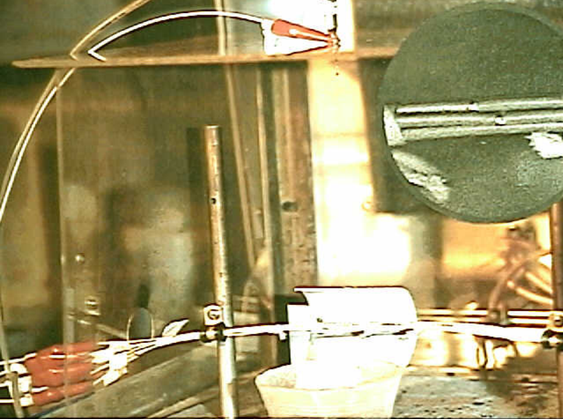
Systems 9 - Electrical Short Circuit/Arcing of Aged Aircraft Wiring - Figure 3. A wire bundle suspended in the wet arc track testing apparatus. (Insert is of the pre-damage cuts in the top wires)..
