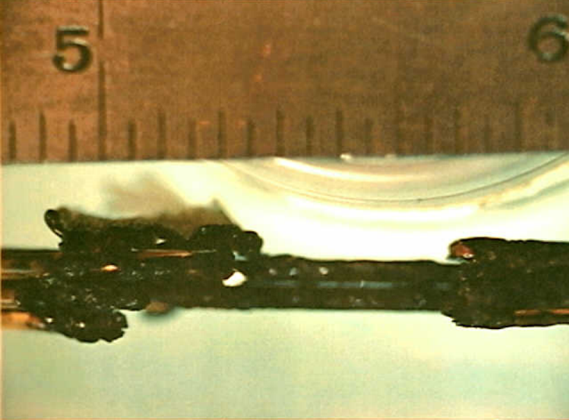
Systems 9 - Electrical Short Circuit/Arcing of Aged Aircraft Wiring - Figure 29. Test 4: Wire bundle after the test including two circuit breaker resets..
