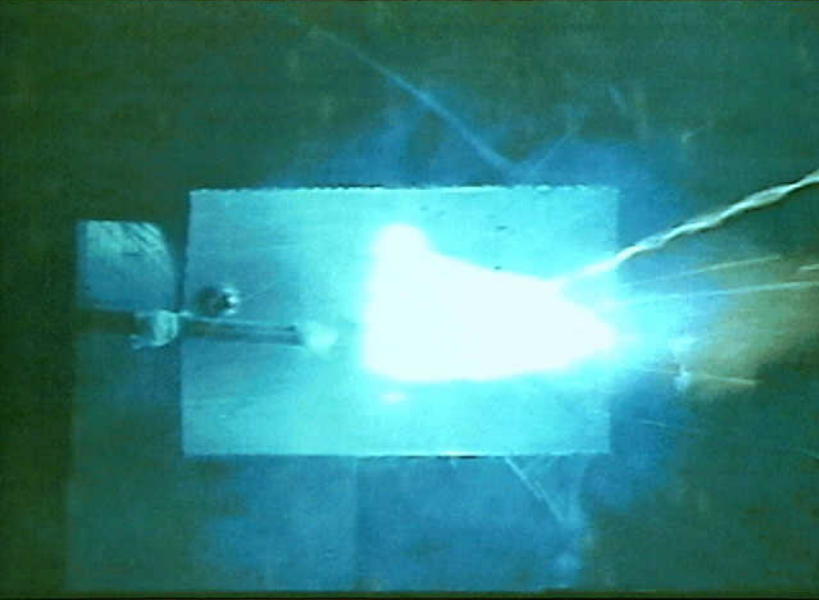
Systems 9 - Electrical Short Circuit/Arcing of Aged Aircraft Wiring - Figure 27. Test 4: Strong arcing on a Mil-W-81381/12-20 wire bundle..
