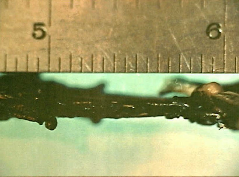
Systems 9 - Electrical Short Circuit/Arcing of Aged Aircraft Wiring - Figure 26. Test 3: Sample bundle after the test which included circuit breaker reset..
