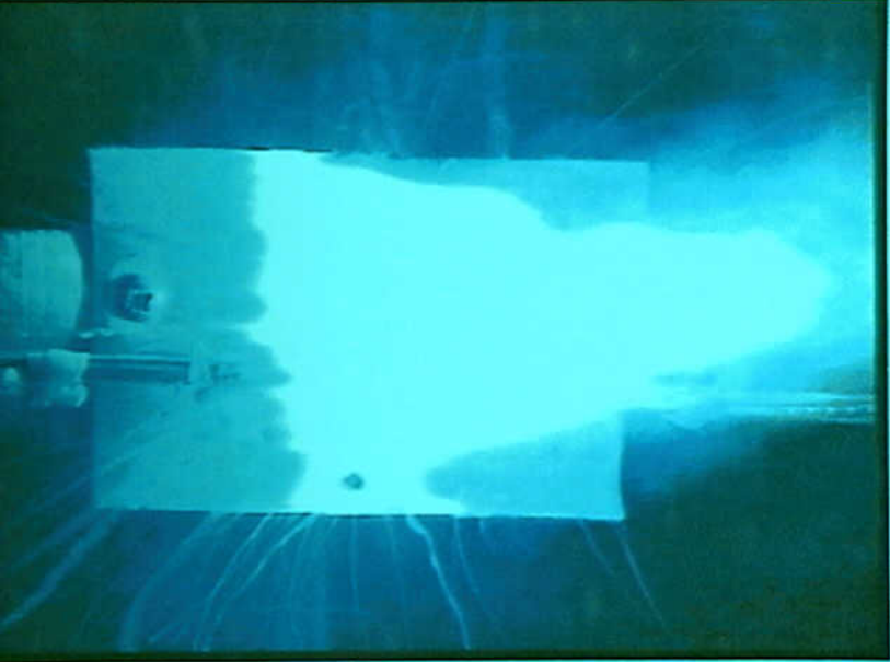
Systems 9 - Electrical Short Circuit/Arcing of Aged Aircraft Wiring - Figure 24. Test 3: Strong arcing on a W42/1/1-20 Sample..
