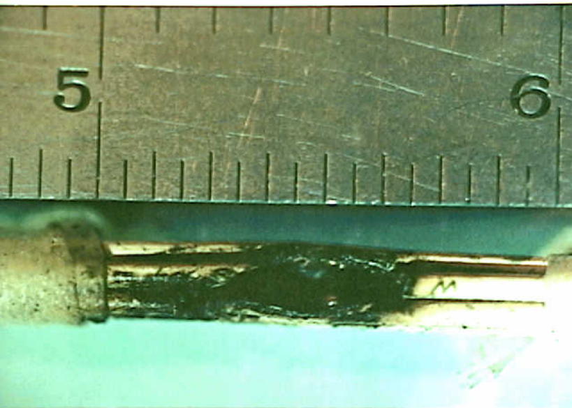
Systems 9 - Electrical Short Circuit/Arcing of Aged Aircraft Wiring - Figure 23. Test 2: Sample bundle after 25 minutes of wet arc track testing..
