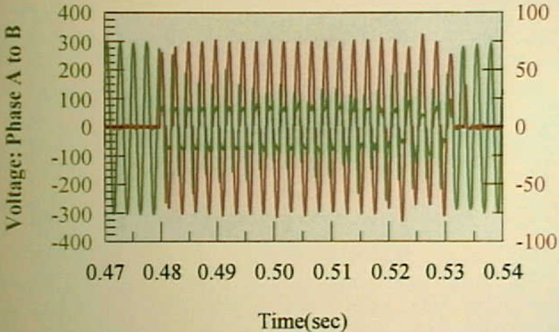
Systems 9 - Electrical Short Circuit/Arcing of Aged Aircraft Wiring - Figure 19. Preliminary Test B: Oscillogram of current during intense flashing event..
