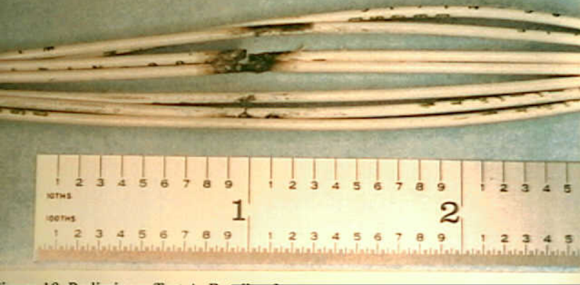
Systems 9 - Electrical Short Circuit/Arcing of Aged Aircraft Wiring - Figure 18. Preliminary Test A: Bundle after wet arc track testing for 5 minutes..
