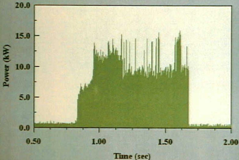
Systems 9 - Electrical Short Circuit/Arcing of Aged Aircraft Wiring - Figure 17. Power in strong arcing event, extrapolated from two phase measurement.
