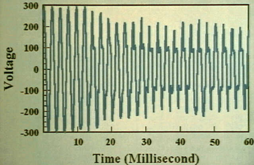
Systems 9 - Electrical Short Circuit/Arcing of Aged Aircraft Wiring - Figure 16. Oscillogram of voltage at the beginning of a strong arcing event..
