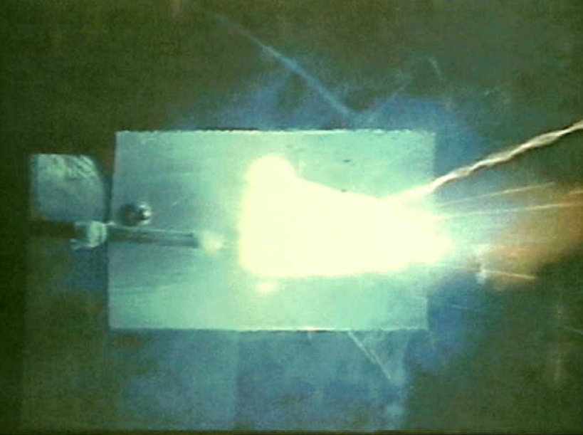
Systems 9 - Electrical Short Circuit/Arcing of Aged Aircraft Wiring - Figure 15. Example of a strong arcing
