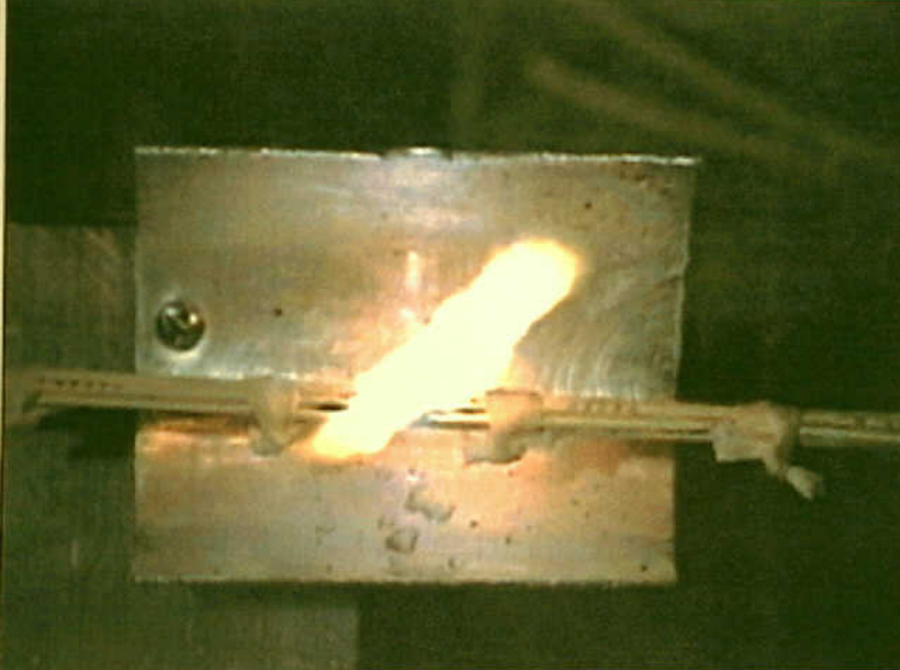
Systems 9 - Electrical Short Circuit/Arcing of Aged Aircraft Wiring - Figure 12. An example of a flashing
