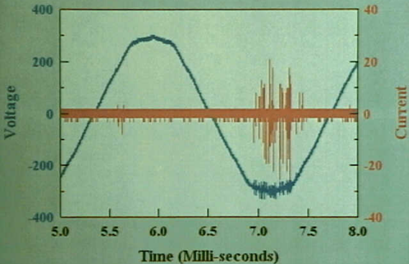
Systems 9 - Electrical Short Circuit/Arcing of Aged Aircraft Wiring - Figure 11. Oscilloscope of voltage from phase A to B (blue ) and current in phase A (red) during scintillations..
