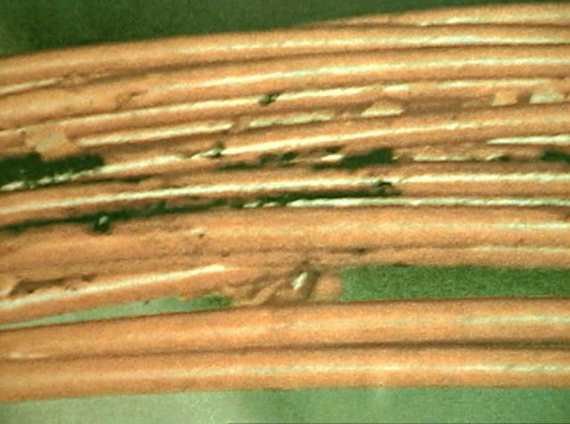
Systems 9 - Electrical Short Circuit/Arcing of Aged Aircraft Wiring - Figure 1. A bundle of Mil-W-81381 wire with visible carbon tracking..
