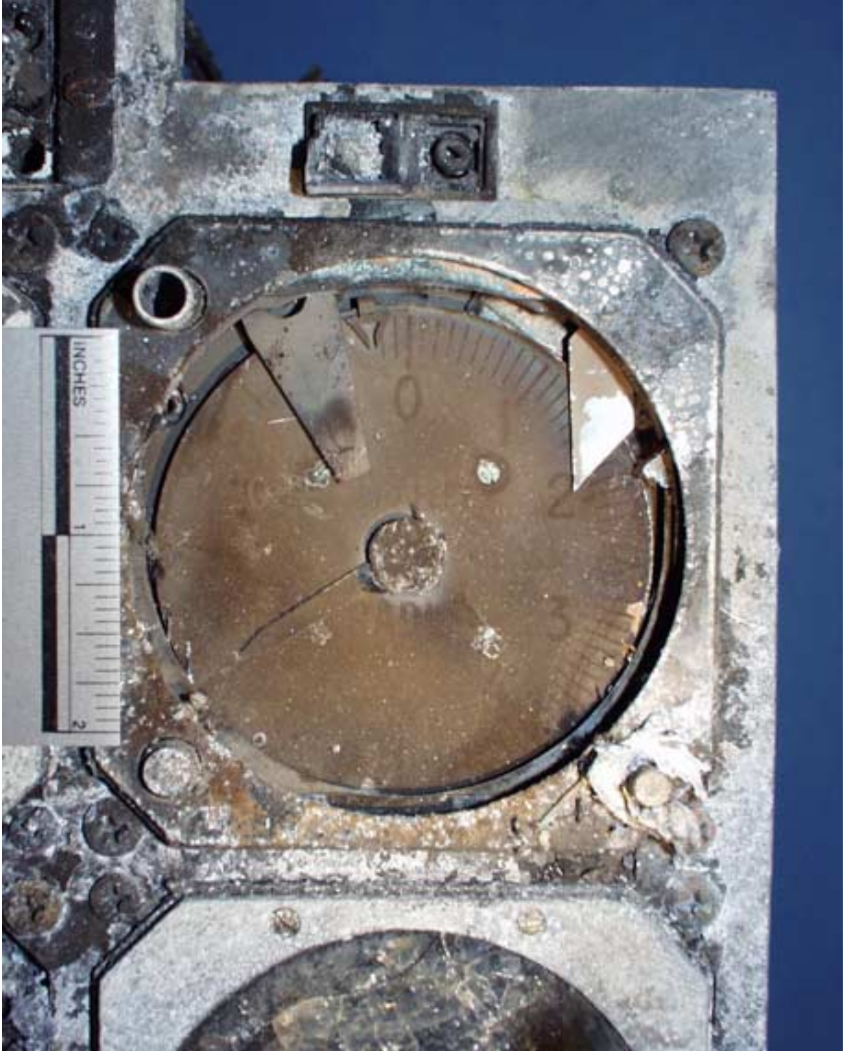
Figure 6-3: Captain's Radio Altitude Indicator
