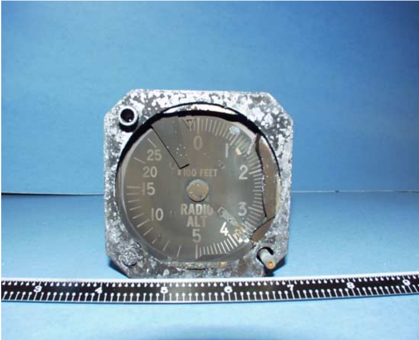
Figure 6-9: First Officer's Radio Altitude Indicator
