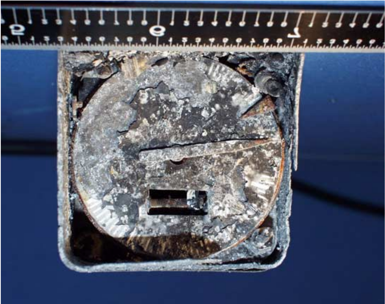
Figure 6-6: Engine Pressure Ratio Indicator, Unknown Engine
