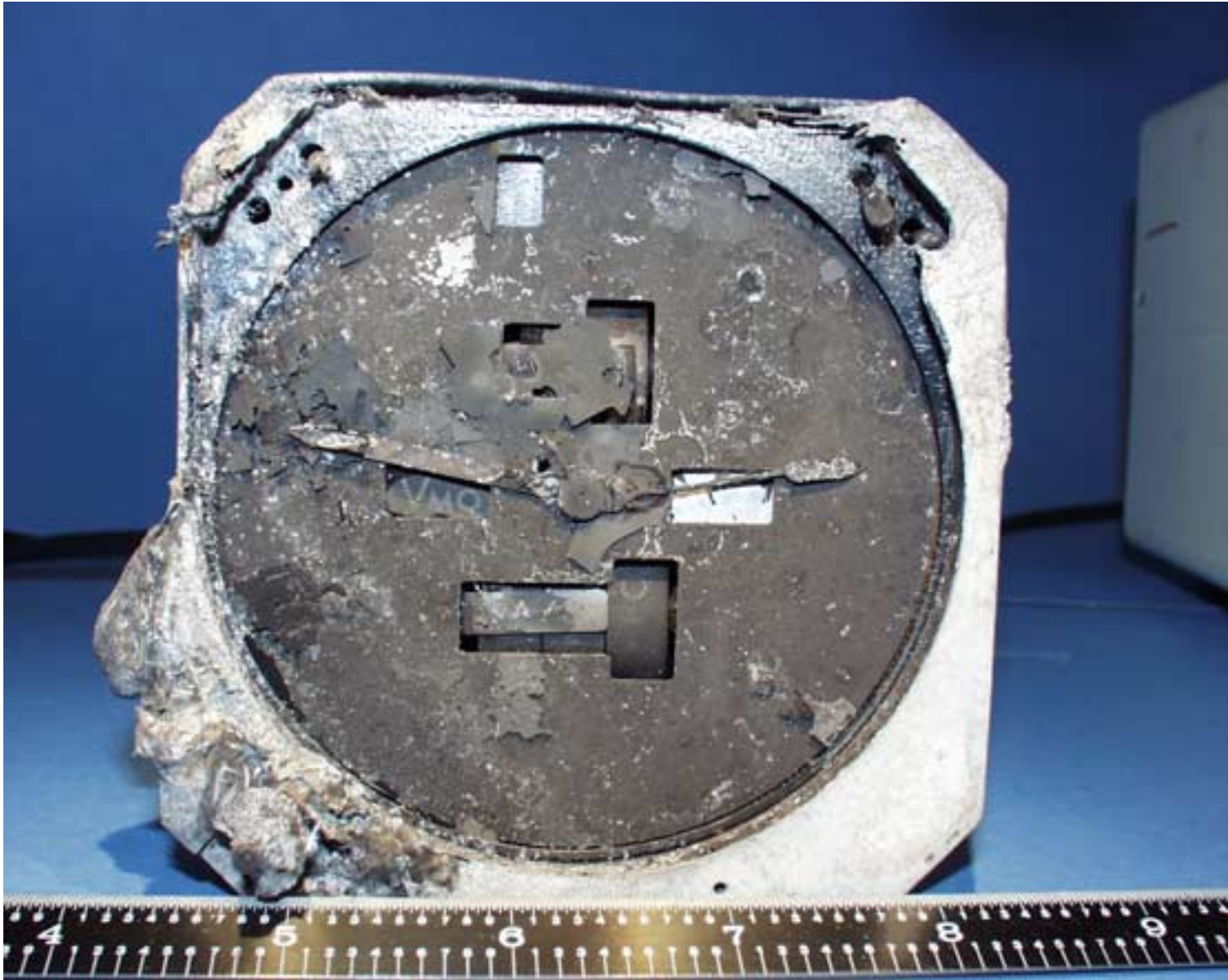
Figure 6-1: Captain's Electric Mach/Airspeed Indicator
