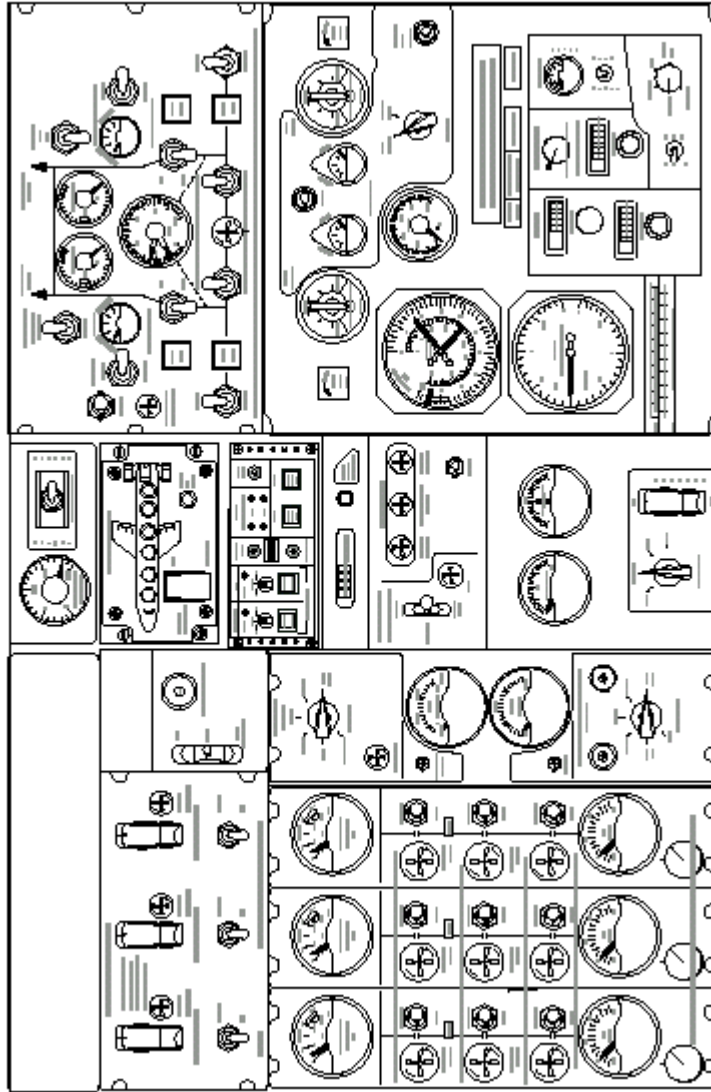
Instrument Panel - Second Officer's Upper - Aircraft 497-499
