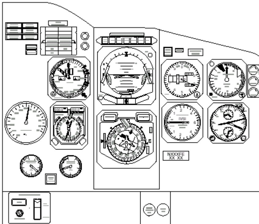
Instrument Panel - First Officer's - Aircraft 497-499
