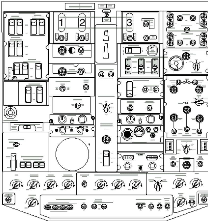
Instrument Panel - Overhead - Aircraft 497-499
