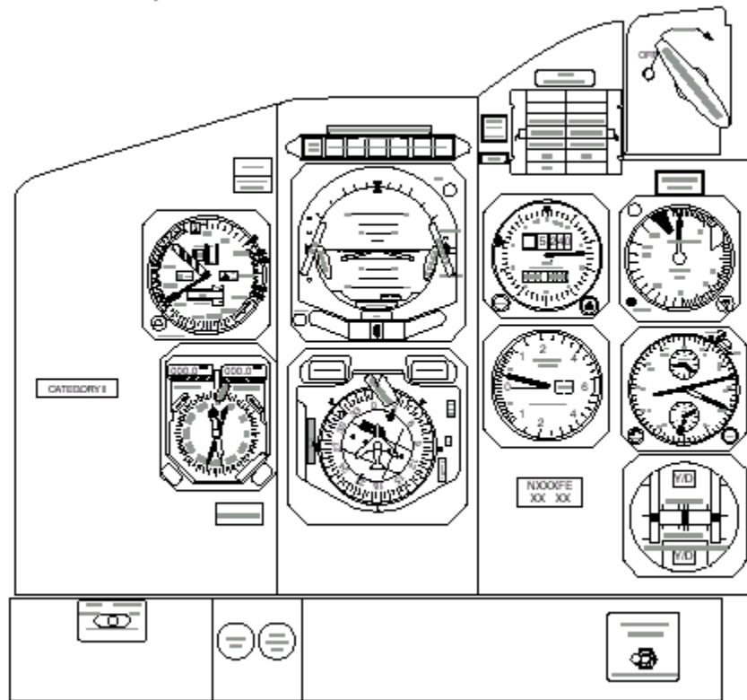
Instrument Panel - Captain's - Aircraft 497-499
