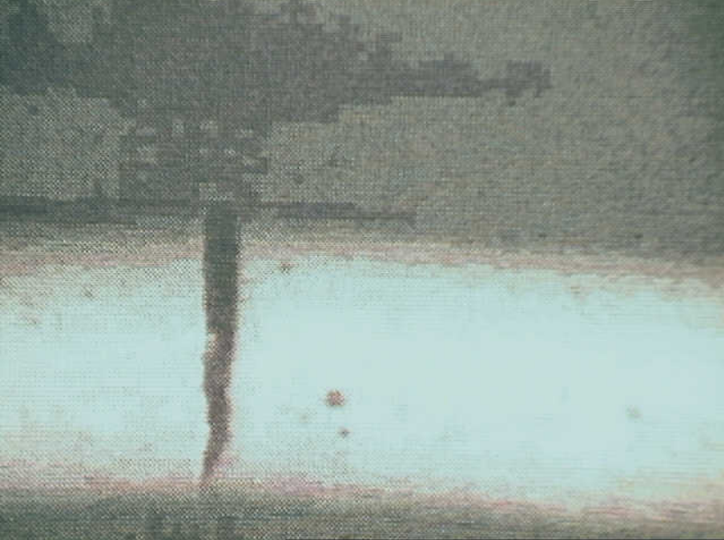
Systems 9 - Aging Aircraft Wire Testing - Photo 3. Radial Cracking (failed dielectric test).
